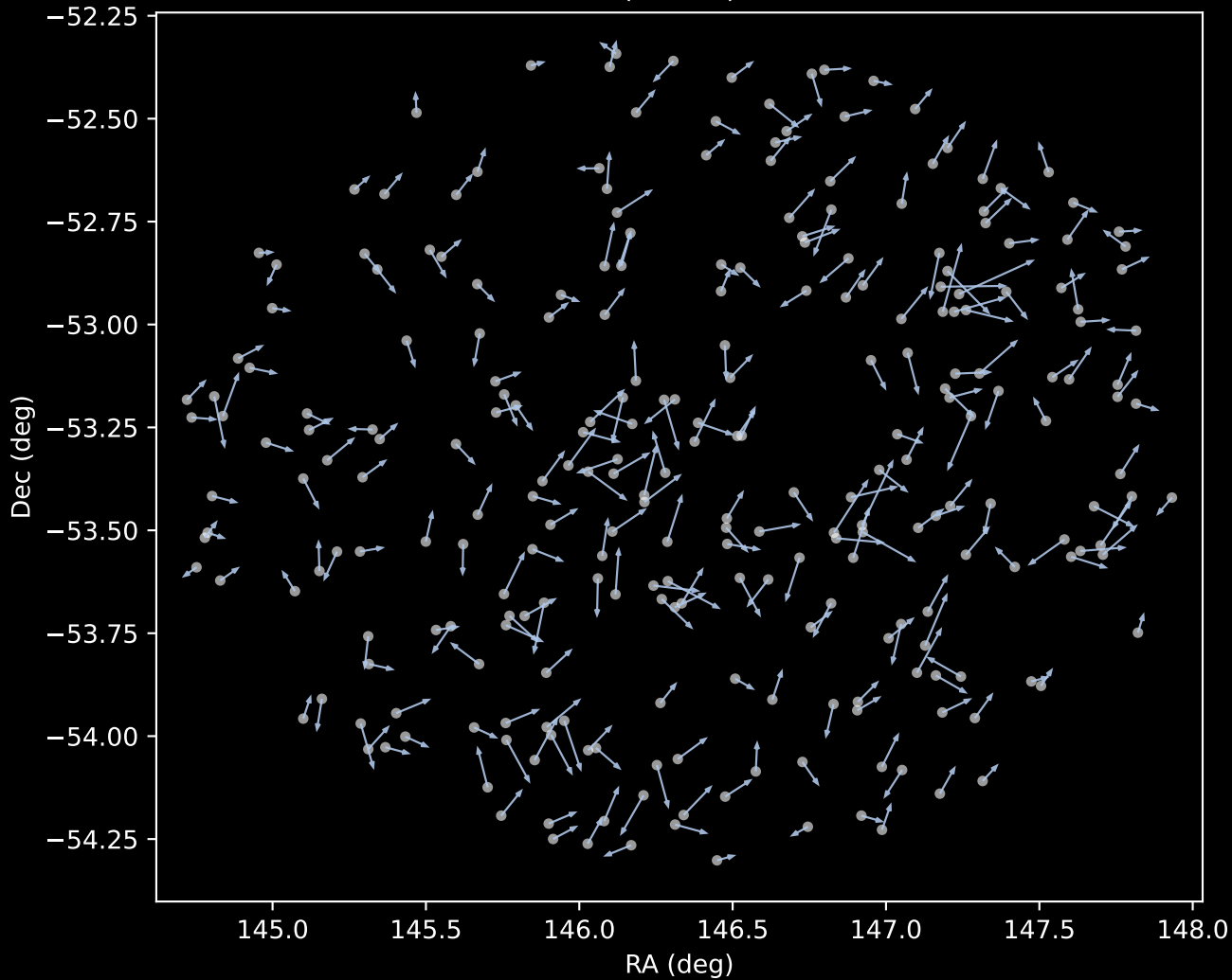
GALAH DR4 Cluster 1 Proper Motion Vectors (n=261)
