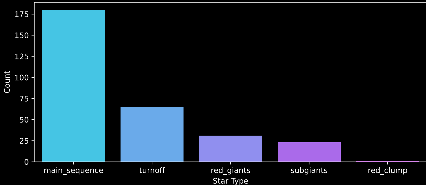
GALAH DR4 Field: [6920] Count plot of Star Type
