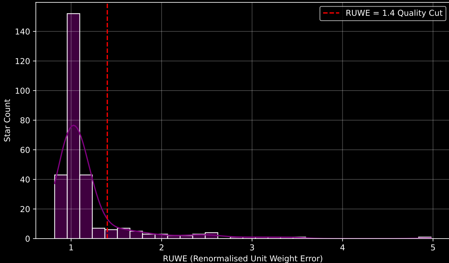
GALAH DR4 Field [6920] RUWE Distribution (n= 287)
